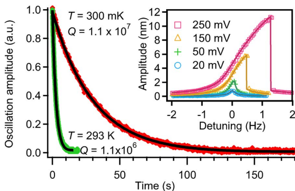
FIG. 2. (Color online) (b) Mechanical ringdown of the membrane. The membrane was driven by a piezoactuator which was stopped at t=0 . Inset shows the nonlinear mechanical response of the Norcada 50 nm membrane. Solid lines are fits.
