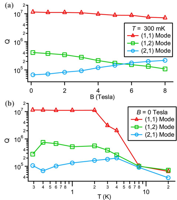
FIG. 3. (Color online) (a) Comparison of Q versus magnetic field ( T=300 mK) for the three lowest vibrational modes of the 50 nm Norcada membrane. (b) Comparison of Q vs temperature ( B=0 ) for the three lowest vibrational modes of the 50 nm Norcada membrane.
