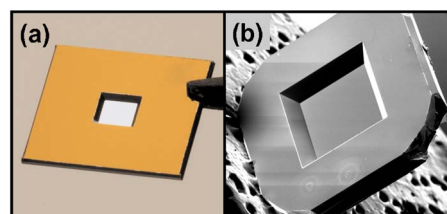
FIG. 1. (Color online) (a) Photograph of a 1 mm × 1 mm × 50 nm Norcada x-ray membrane. (b) SEM of an SPI 1 mm × 1 mm × 50 nm membrane.
