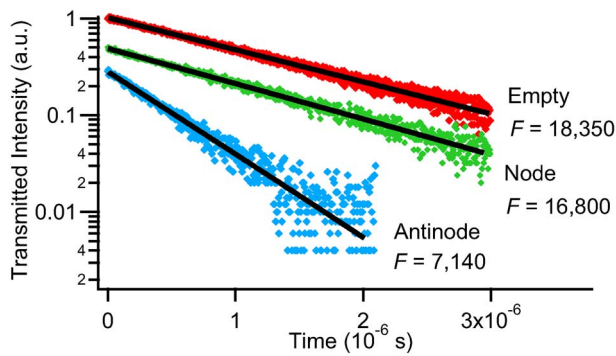
FIG. 4. (Color online) Ringdown of transmission from cavity after the laser is chopped at t=0 , shown with fitted values of finesse.
